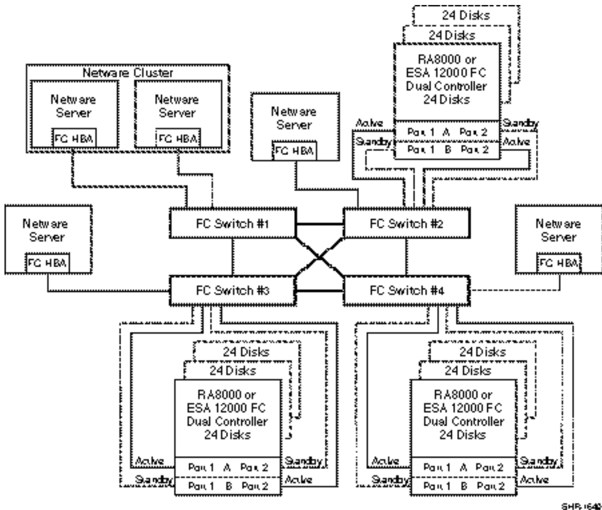
Figure 4 Four Switches, Cascaded Meshed Fabric Configuration Example
