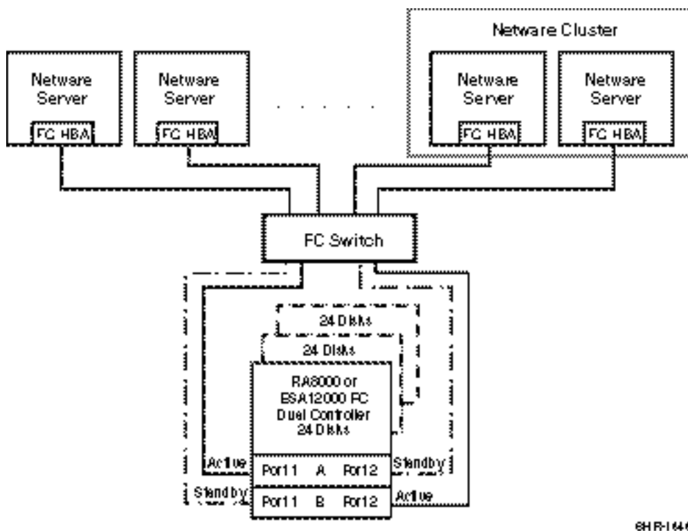
Figure 1 One Switch Fabric Configuration Example
