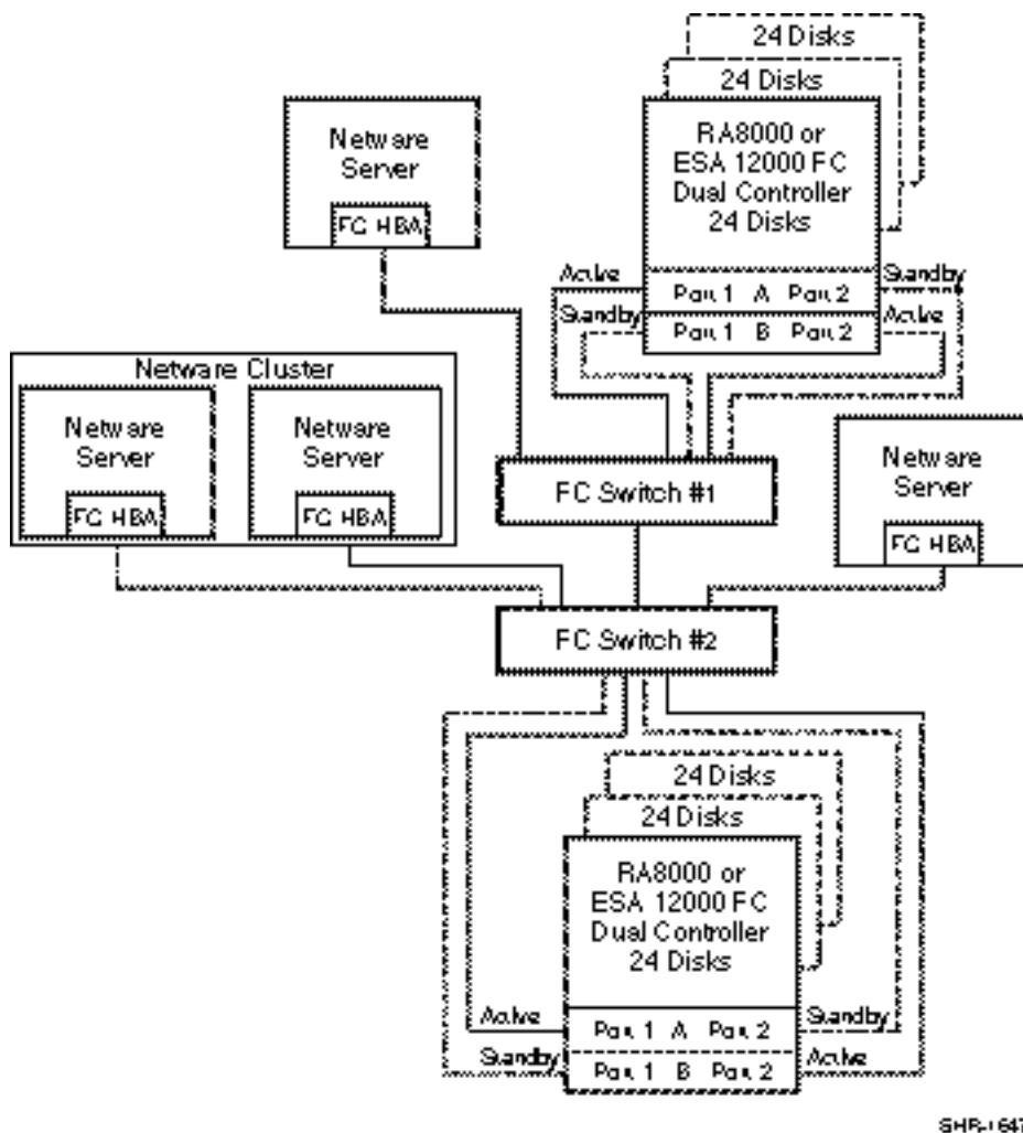
Figure 2 Two Switches, Cascaded Fabric Configuration Example
